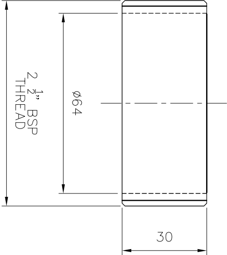
(SCALE-1:4) DETAIL-A BUSH FOR COUPLER
